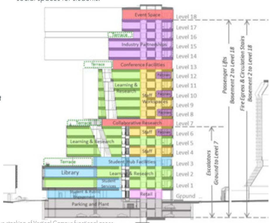
Figure 5. Section Diagram showing indicative stacking of Vertical Campus functional zones
