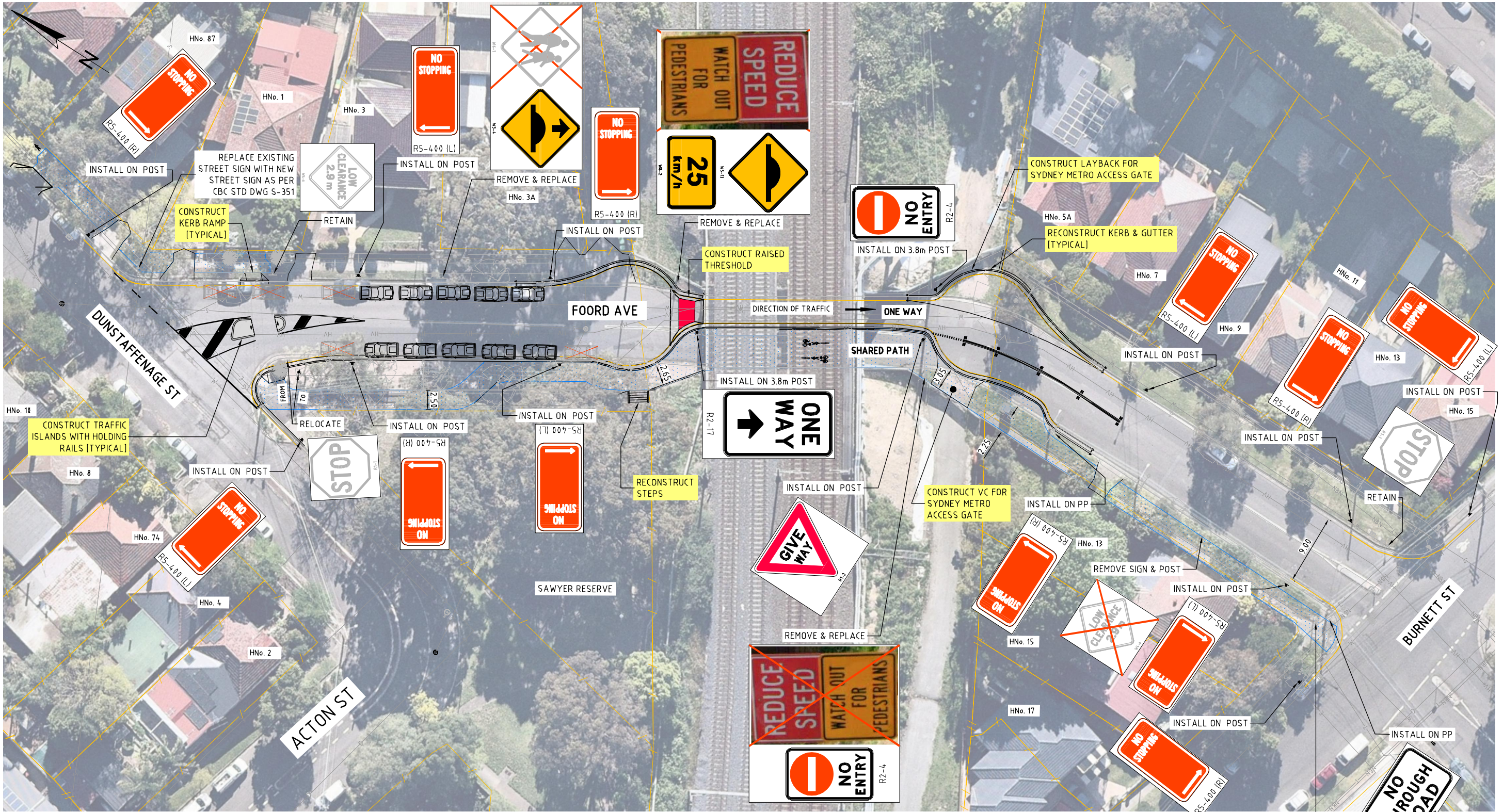
GENERAL ARRANGEMENT PLAN SCALE 1:500
