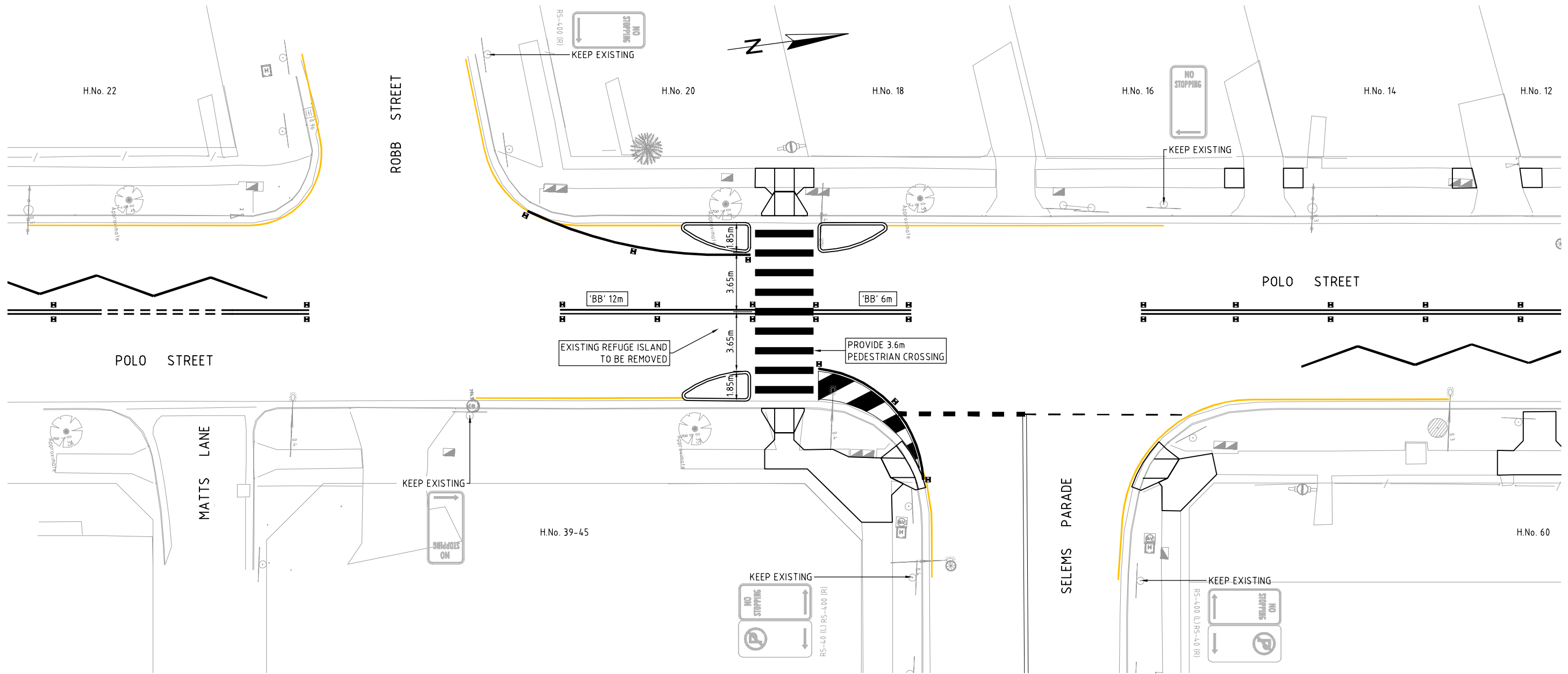
LINE MARKING PLAN SCALE 1:250
