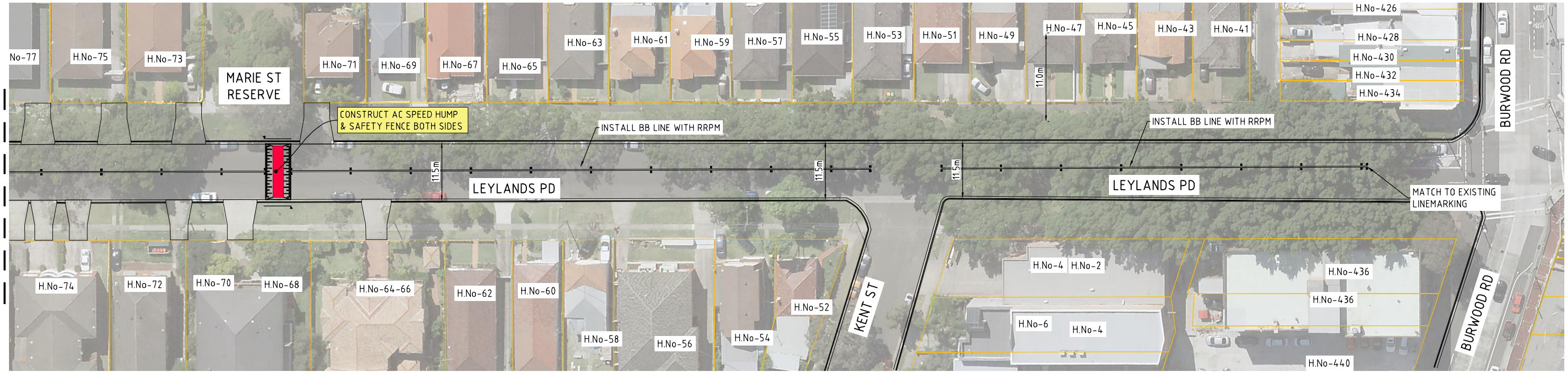
SPEED HUMP ARRANGEMENT PLAN SCALE 1:1000
